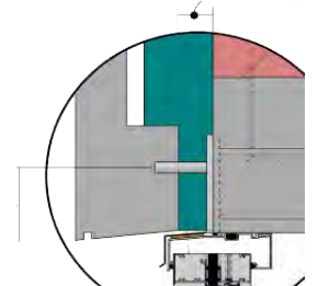
Stainless Steel Clip Mount: Lateral Connection Detail
