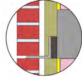
Insulation covers shelf angle for scenarios R-10+
