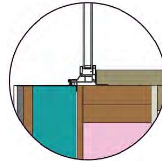
Sill Detail
