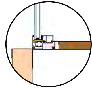
Sill Detail
