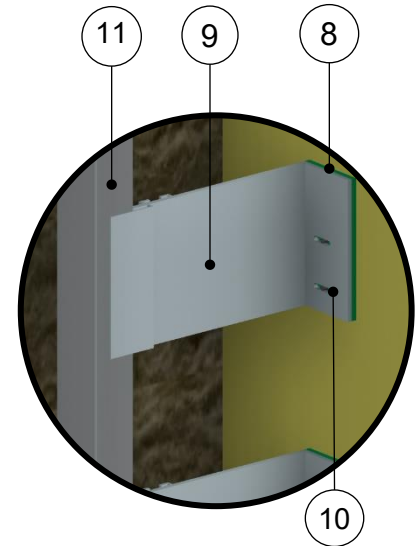
Nvelope NV1 Clip Detail
