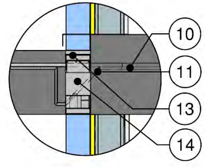
Isokorb K65-V8 Detail
