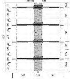
Isokorb KXT15-V6 Rebar Arrangement
