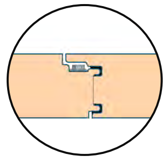
Vertical Joint
