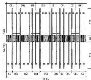
Isokorb K65-V8 Rebar Arrangement
