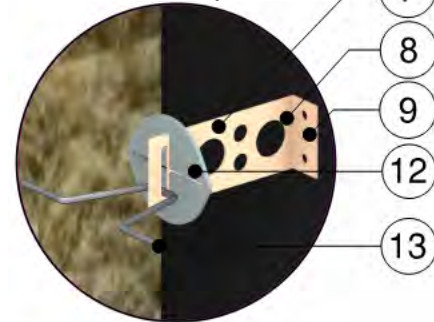
Slotted Rap-Tie with Aerogel Coating
