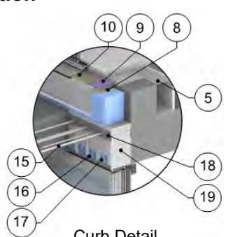
Curb Detail
