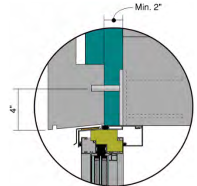
Stainless Steel Clip Mount: Lateral Connection Detail
