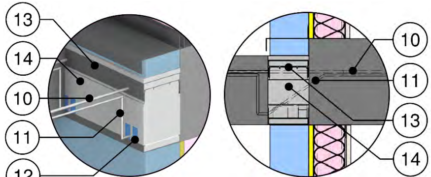
Isokorb K10-V6 Detail
