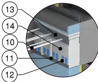
Isokorb K65-V8 Detail
