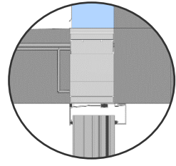
Scenario A - Window wall thermal break located at concrete slab, un-insulated glazing frame
