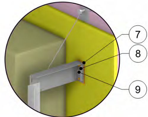
Console Detail
