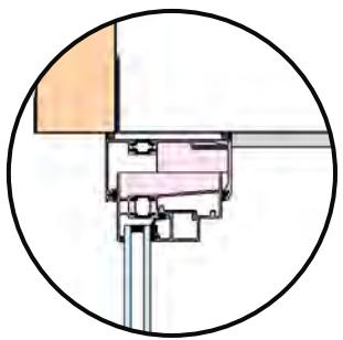
Head Detail
