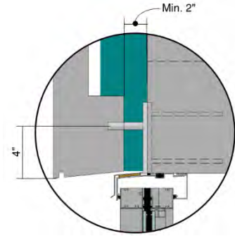
Stainless Steel Clip Mount: Lateral Connection Detail
