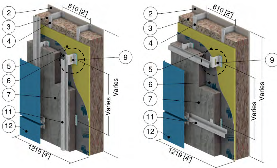
Vertical Girt: ACS Clip Detail
