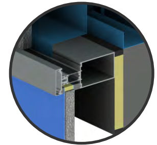
F2 – Rigid Insulation Spacer, 1" (25 mm) AIM between Metal Skins
