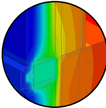
Mullion Detail
