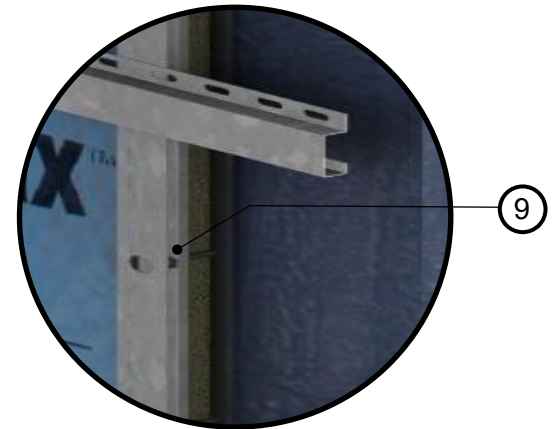
Isolator Detail
