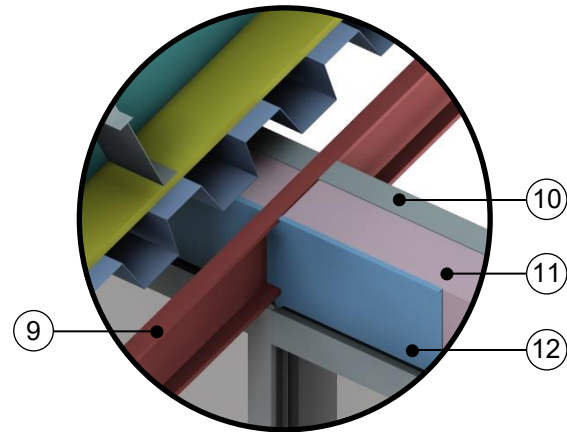
Through Beam and Metal Deck at Curtain Wall
