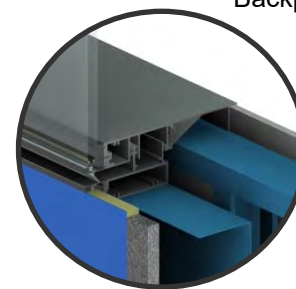
H3 – Rigid Insulation Spacer, 1" (25 mm) AIM between Metal Skins
