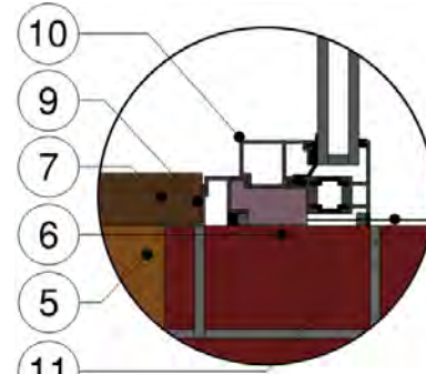
Case A: Window on Brick with Insulation at Window Perimeter
