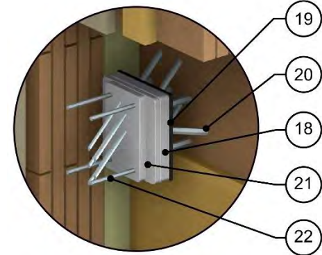
Connector Detail
