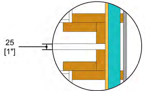
Fire Wall and Exterior Wall Intersection Detail
