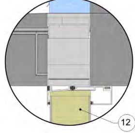
Scenario B - Window wall thermal break located at Isokorb module, insulated glazing frame
