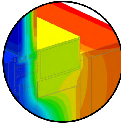
Mullion Detail
