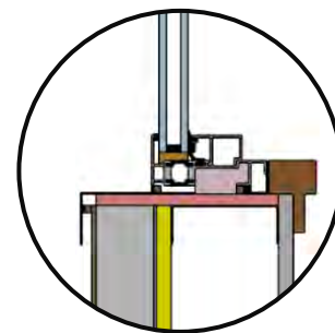
Sill Detail
