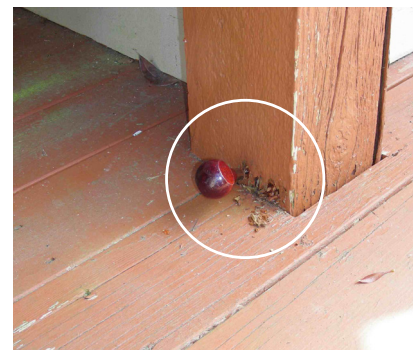
Probe reveals deteriorated wood post masked by solid stain
